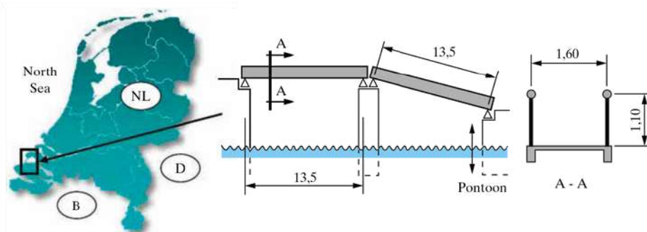
Fig. 2: Bridge location and dimensions (Units: m)
