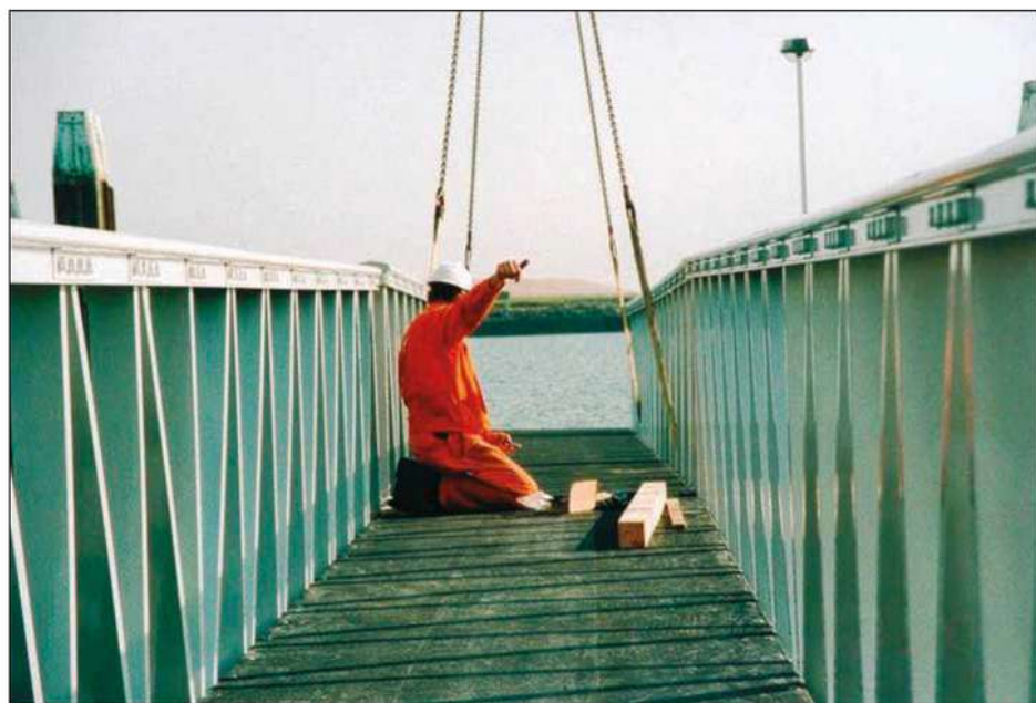
Fig. 1: Installation of the Noordland inner harbour footbridge
