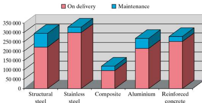
Fig. 4: Energy impact of the bridge for the five material options
