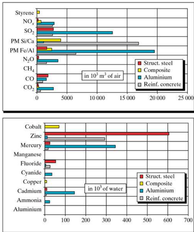
Fig. 5: Polluted air and water as a result of bridge construction with four material options
