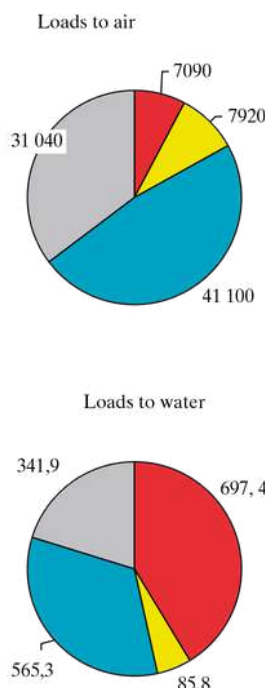
Fig. 5: Polluted air and water as a result of bridge construction with four material options
